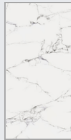
Shale
